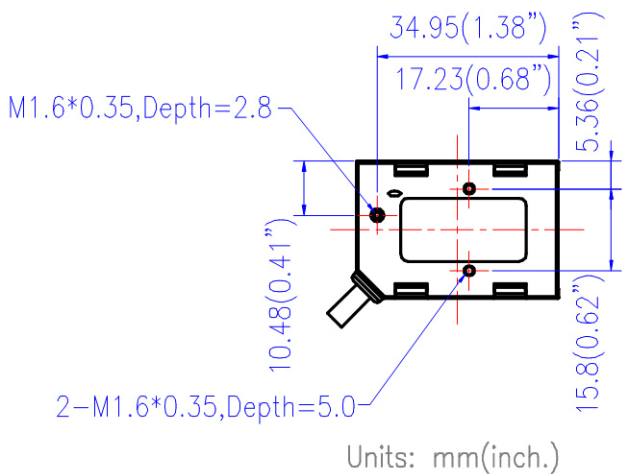
Figure 1: Screw Position
