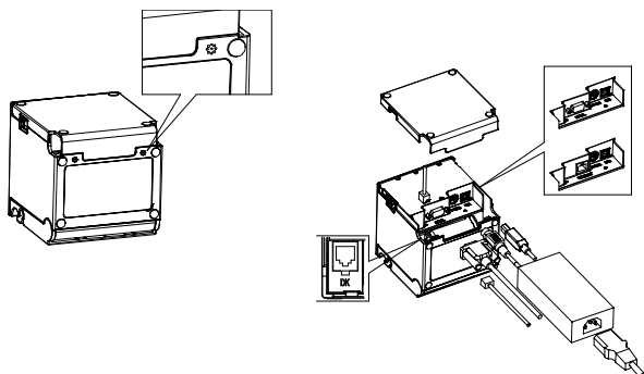
Paberi paigaldamine 1
