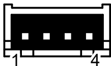
POWER SUPPLY JST male connector (S4B-PH-K-S)
